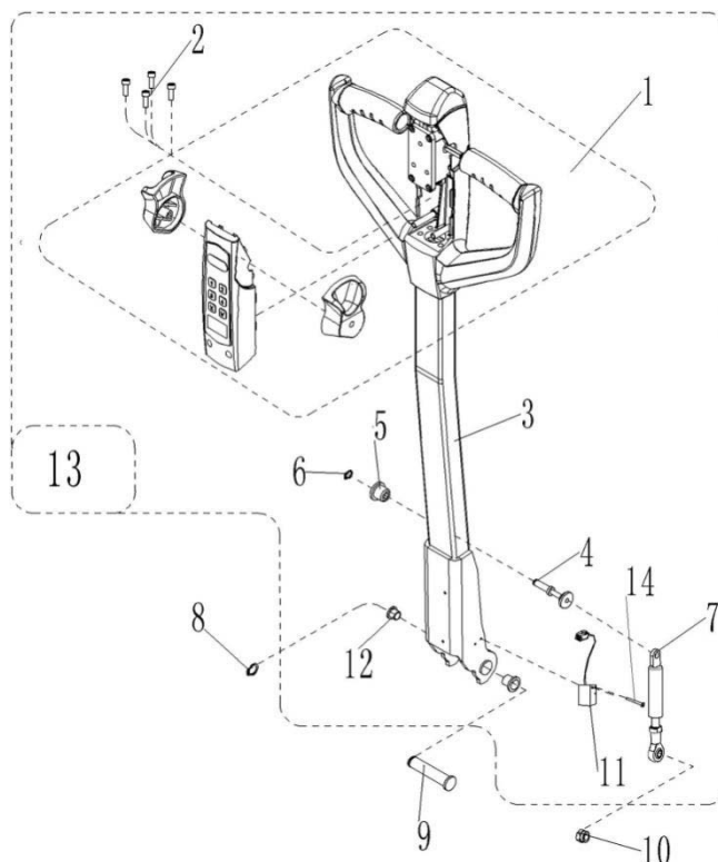
Fig. 12 Tiller Arm Components
