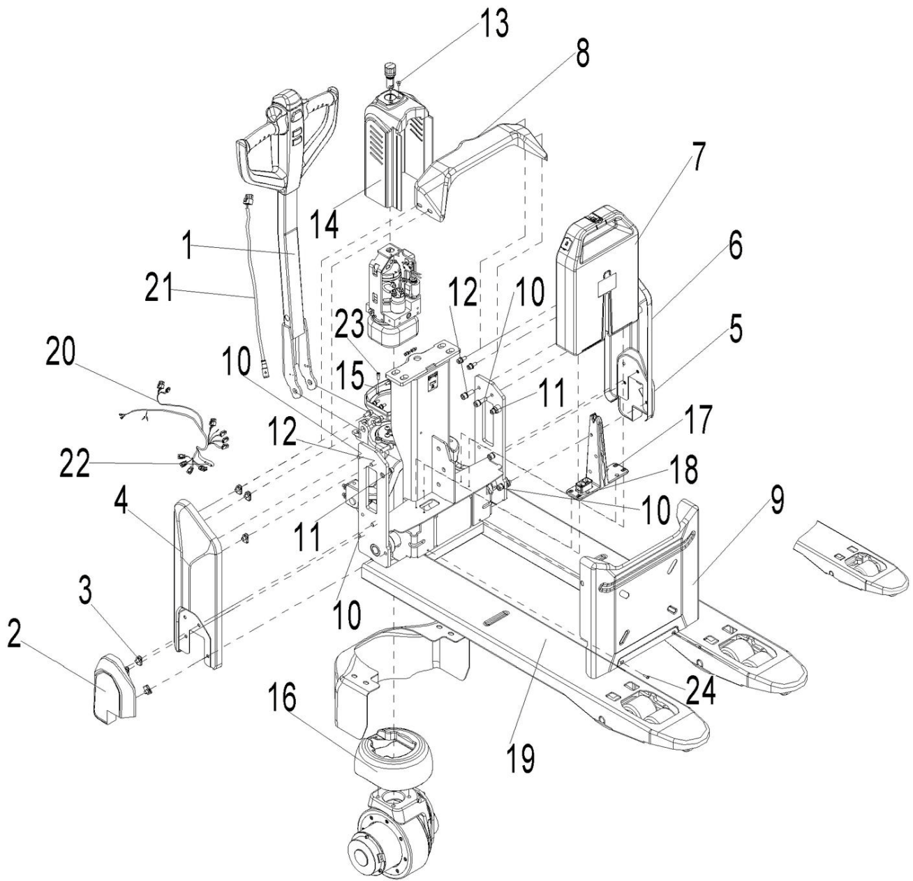
Fig. 13 Truck components
