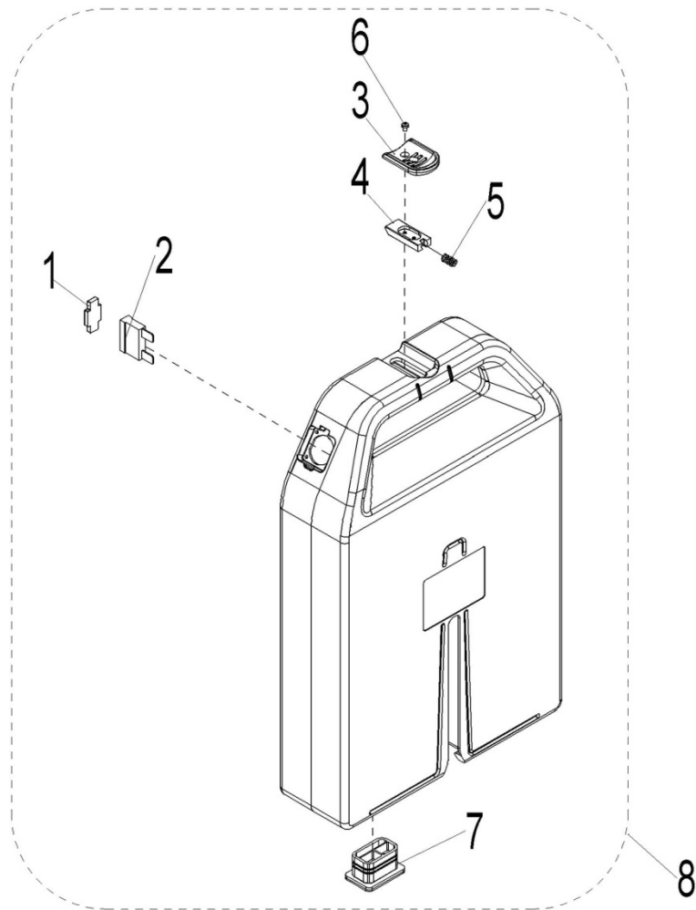
Fig. 14 Power Supply Assembly
