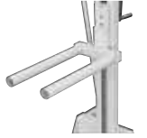
Art. no E-DS Diameter = Ø 47 mm Length = 450 mm CC distance = 200 mm
