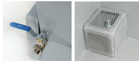
Net - crane – tight welding for liquid separation
